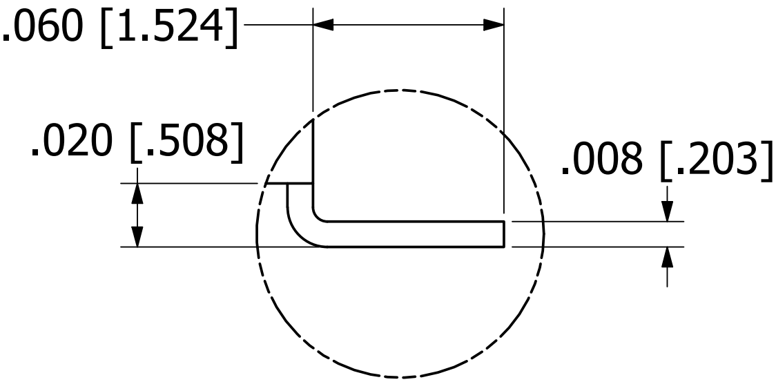
DETAIL A
